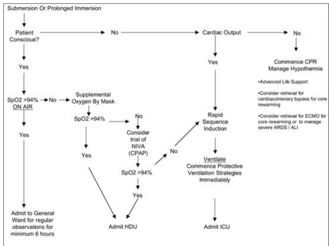
Fig 3. Treatment Algorithm
